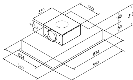
Ceiling Stripe 90 SM
